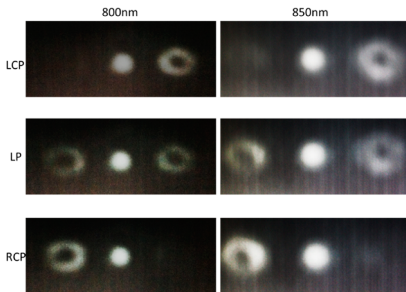
Figure 7. Captured infrared images of the transmitted diffraction patterns from the gradient-rotation array sample with 15^\circ gradient step at 800 and 850 nm under the incident beams with left-handed circular polarization, linear polarization, and right-handed circular polarization, respectively.
