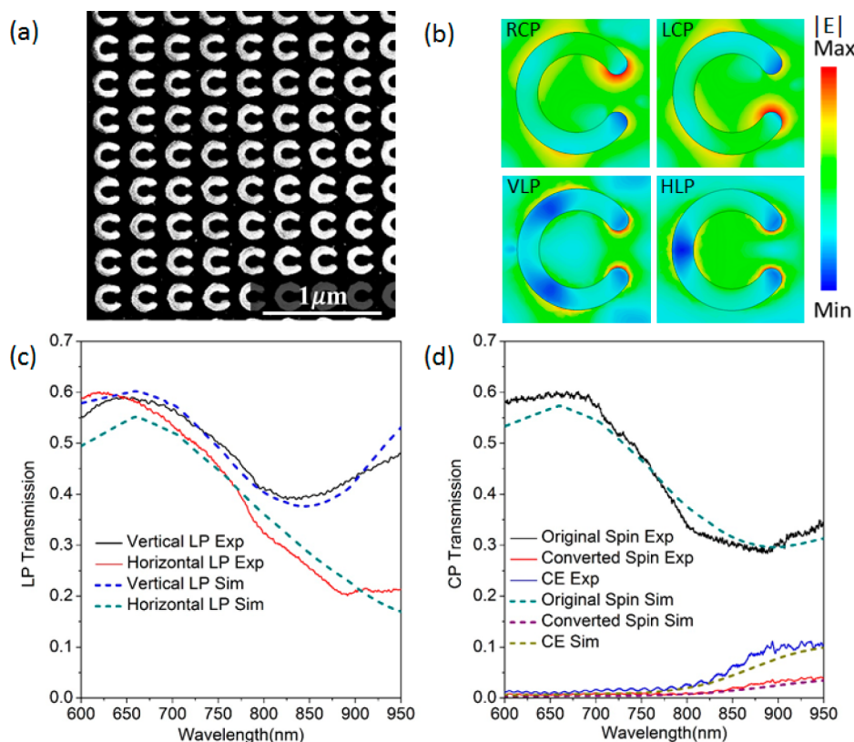
Figure 2. (a) One SEM image of the fabricated split-ring antenna homogeneous array. (b) Simulated optical field |E| distributions of split-ring antennas under orthogonal polarizations at 900 nm. (c,d) Measured and simulated transmission spectra under linear polarization basis and circular polarization basis, respectively.
