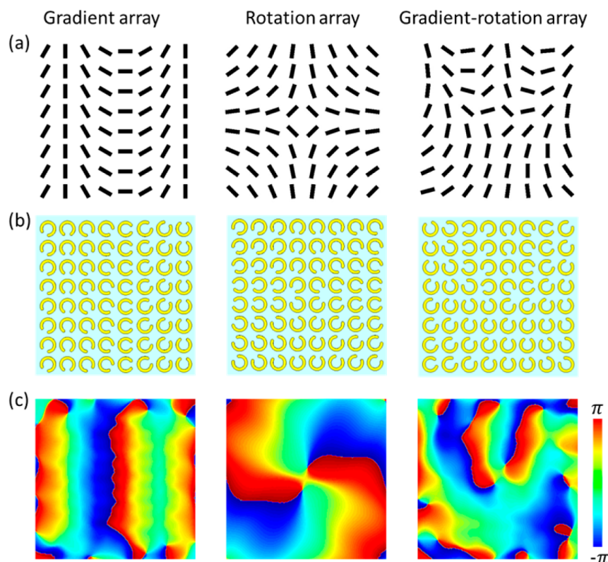
Figure 3. (a) Schematics of the optical axis orientation distributions of split-ring antennas for gradient array, rotation array, and gradient-rotation array, respectively. (b) The corresponding split-ring antenna arrays. (c) Simulated near-field phase distributions of the converted spin components from these inhomogeneous antenna arrays.
